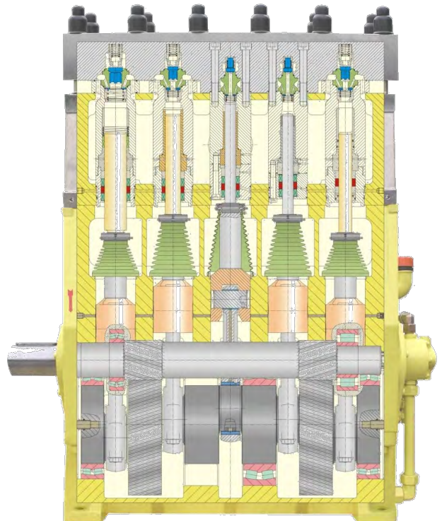
view showing a range of sealing options
